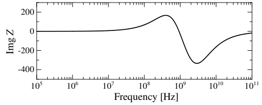
(b) Imaginary part impedance.
