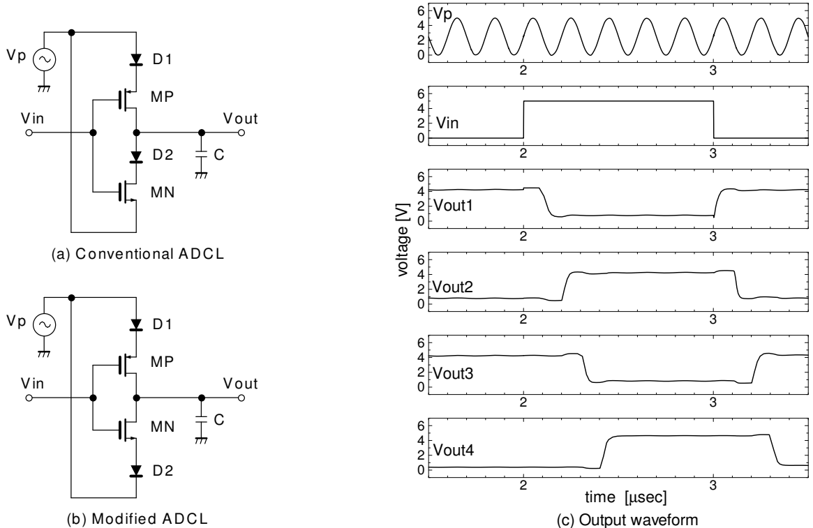
Figure 1: Adiabatic dynamic CMOS logic (ADCL) and simulated waveform of four ADCL inverter-chains.
