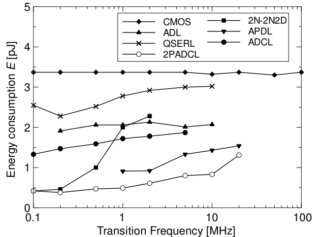
Figure 3: Energy consumption of different diode based adiabatic logics and CMOS logic.
