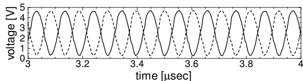
Figure 5: Output voltages of the adiabatic power supply circuit.
