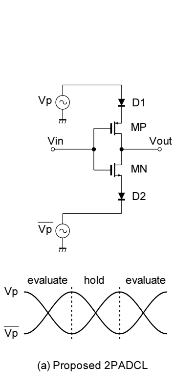
Figure 2: Two-phase drive ADCL (2PADCL) and simulated waveform of chain of four 2PADCL inverters.
