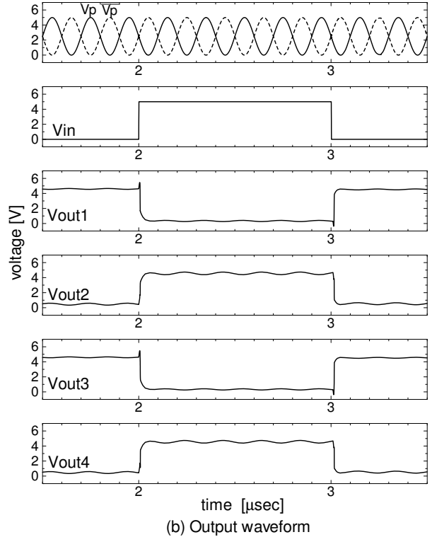
Figure 2: Two-phase drive ADCL (2PADCL) and simulated waveform of chain of four 2PADCL inverters.
