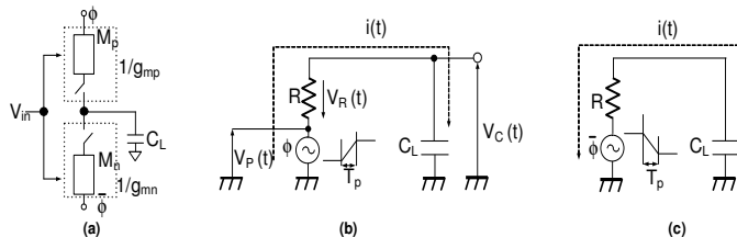
Fig. 2. (a) Model of adiabatic logic showing an ideal switch in series with resistance and two complementary voltage supply clocks. (b) Charging activity. (c) Discharging activity.
