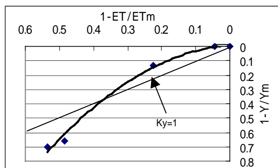
Figure 1. The relation between relative decreased ( 1-Y_a/Y_m ) and relative ET ( 1-ET_a/ET_m )
